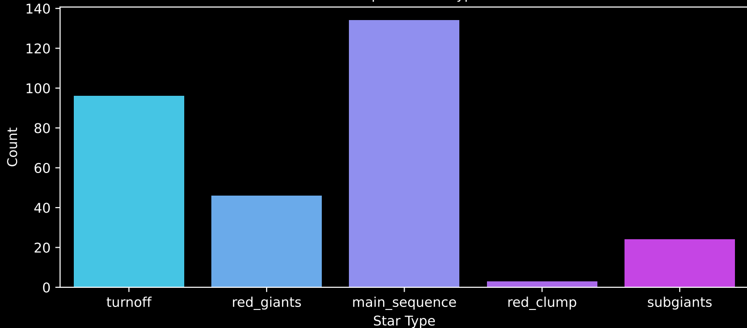
GALAH DR4 Field: [1173] Count plot of Star Type
