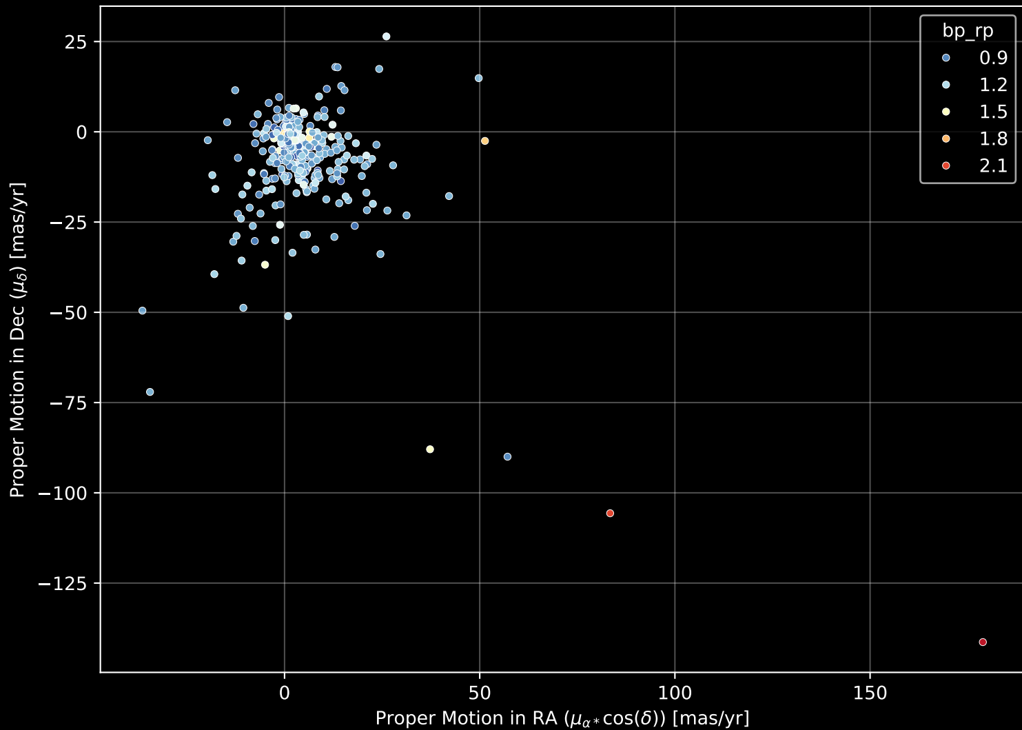
GALAH DR4 Field: [1173] Proper Motion Diagram (n= 303)
