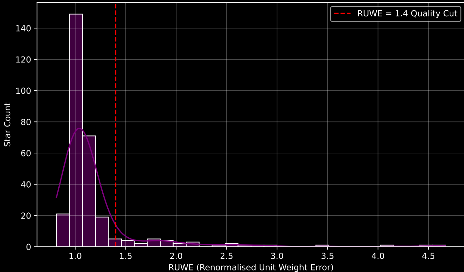
GALAH DR4 Field [1173] RUWE Distribution (n= 295)
