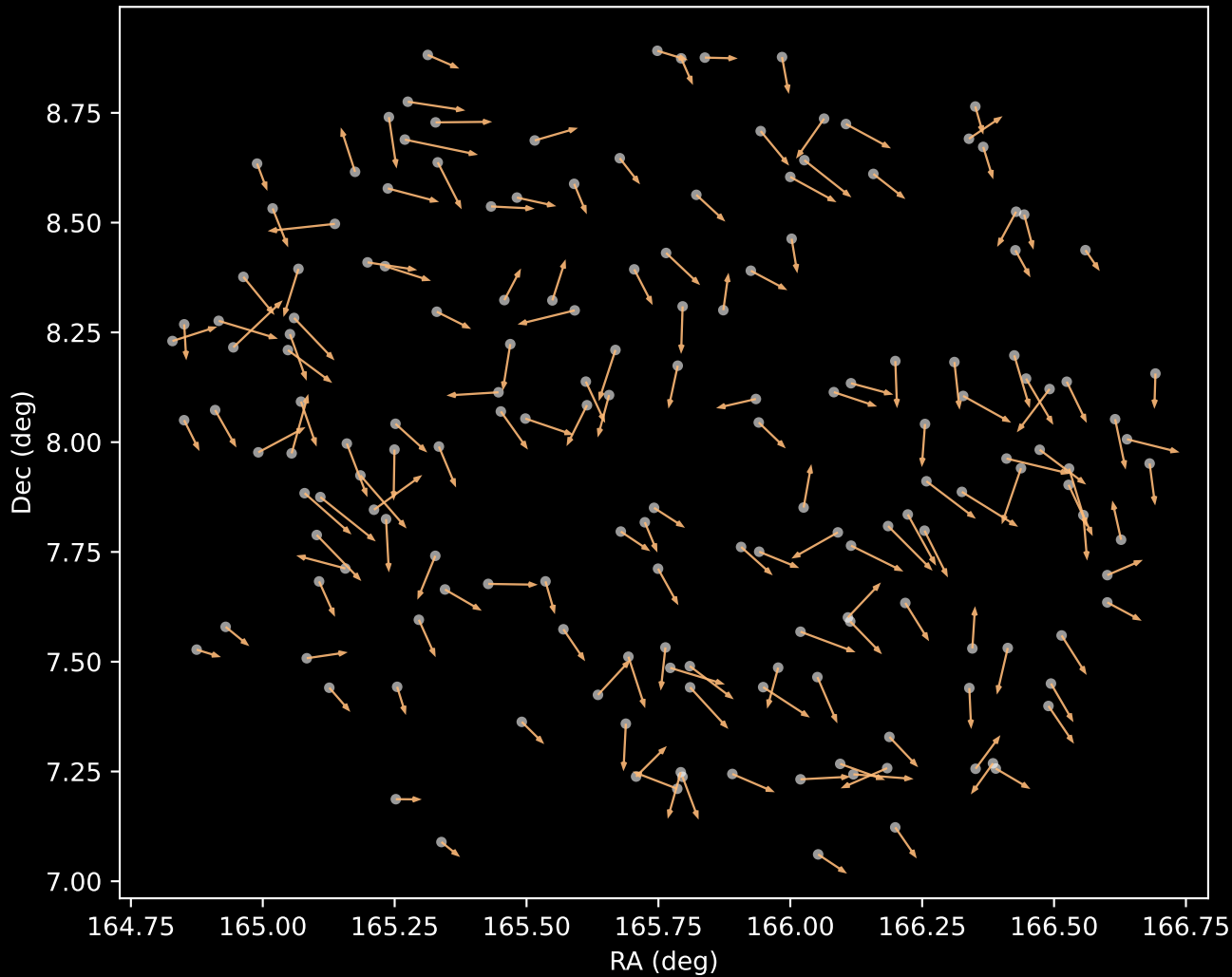
GALAH DR4 Cluster 3 Proper Motion Vectors (n=169)
